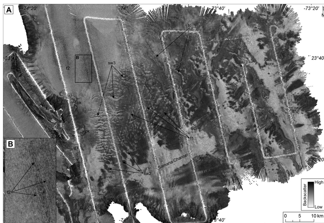
Fig. 12. Enlargement of the backscatter image of the San Salvador turbidite system. Low reflectivity corresponds to light tones; high reflectivity corresponds to dark tones. f1, f2: furrows; pk: pockmarks; sw2 and sw3: sediment waves; tc: tension cracks. B: Enlargement of the map showing furrows f2. See Fig. 1B for location.
